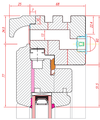
Lipped Head Section
