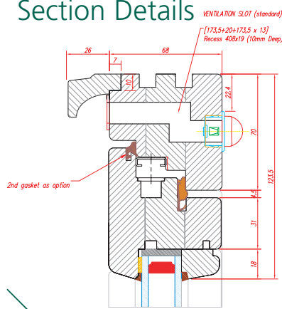
Flush Head Section
