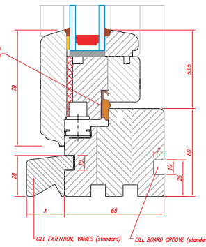
Lipped Sole Section
