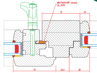
Mullion Section
